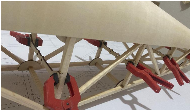
12) Glue pull-pull rods fixing seat.
